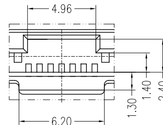
VIEW 0 SCALE 2:1
