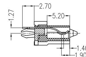
SECT B-B
